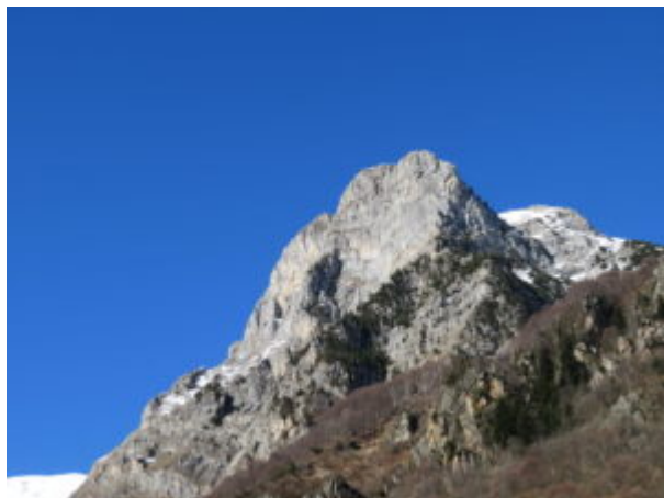
Cima Cars
